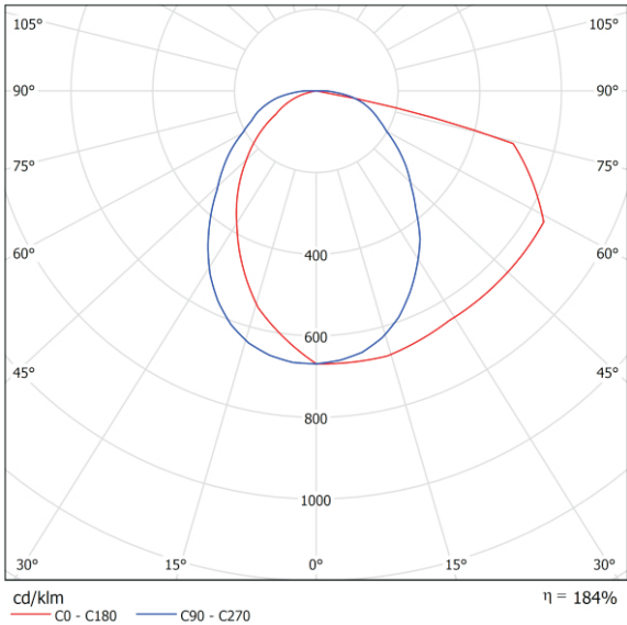
Light Distribution Pattern
